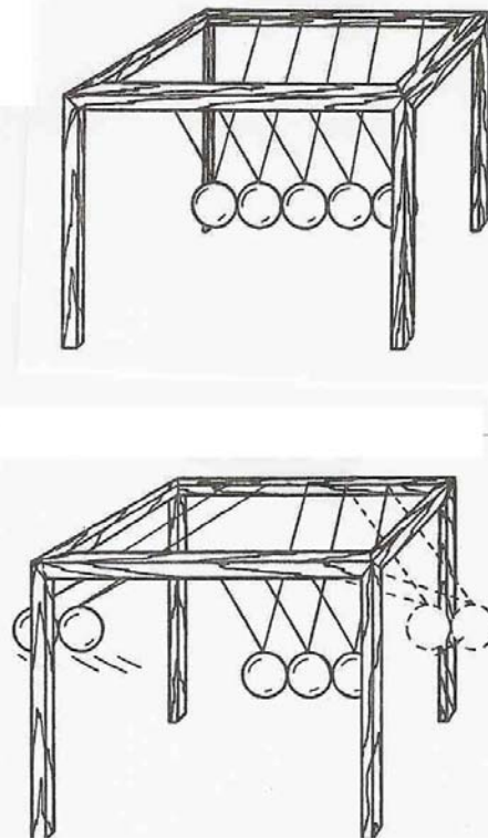
Figure 2. The Energy-Momentum Toy
